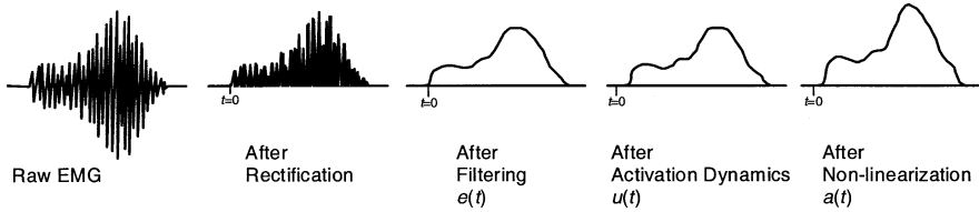
Figure 3 — Muscle activation dynamics: Transformation from EMG to muscle activation.
