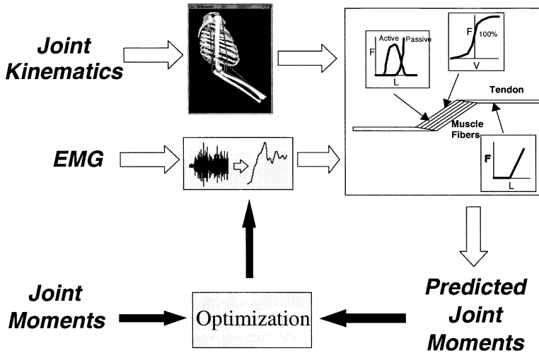
Figure 8 — Flowchart of the modeling procedure. EMG is processed to obtain muscle activation while the position data is used to obtain musculoskeletal lengths, velocities, and moment arms. Together these are put into a Hill-type model to estimate musculotendon forces, and these in turn are multiplied by their moment arms and summed to obtain joint moment. This estimated moment is compared with the measured moment. In the optimization process, parameters in the model are adjusted to minimize the difference between measured and predicted joint moments. Once the parameters are tuned, the optimization part of the model is removed and it can now be used to predict joint moments for novel tasks.
